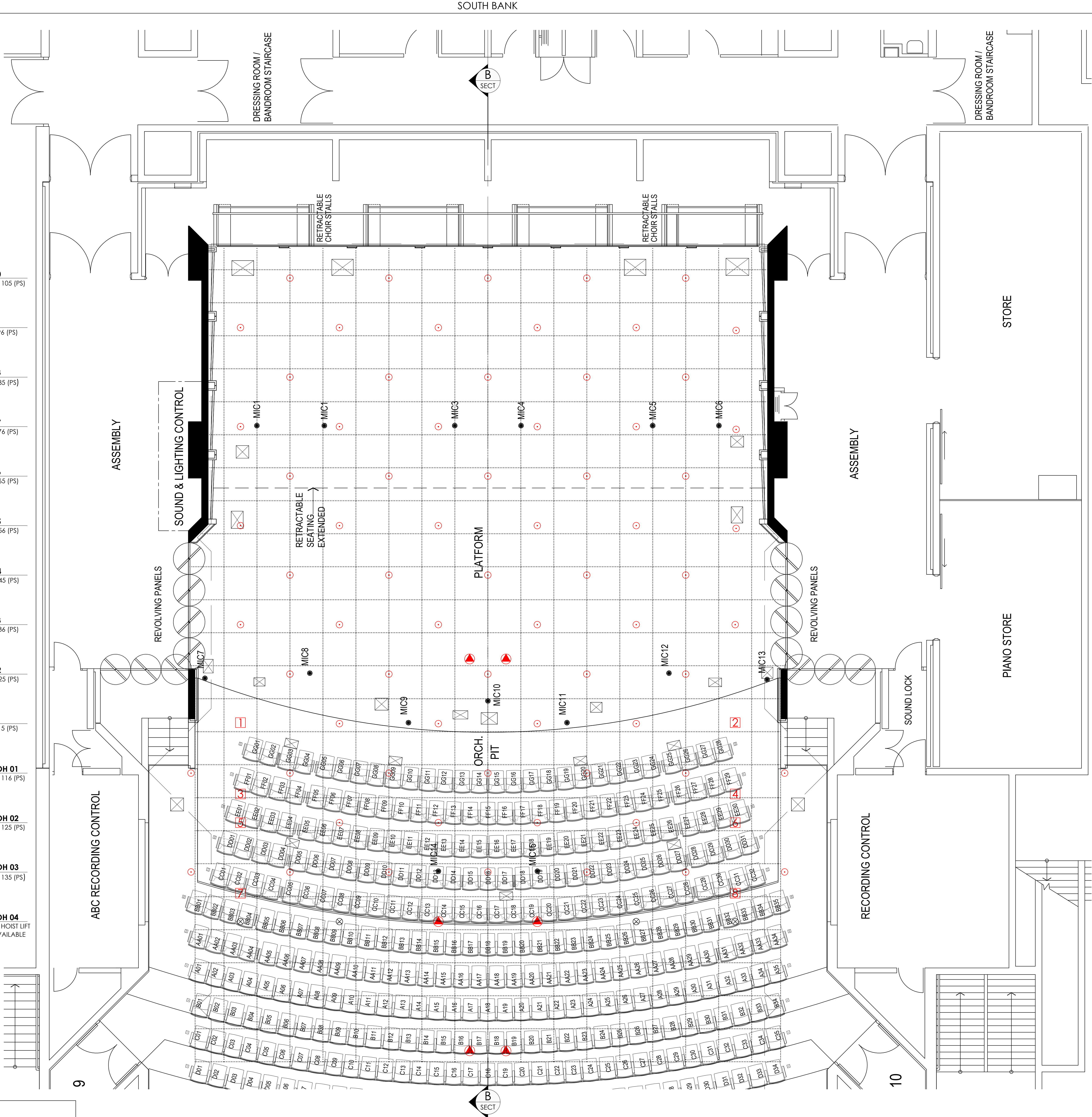
CONCERT HALL PLATFORM PLAN SHOWING CEILING OVERLAY SCALE = 1:50 @ A0 SCALE = 1:100 @ A2
